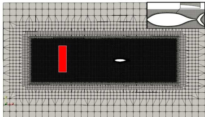
Figure 2. Numerical mesh.
