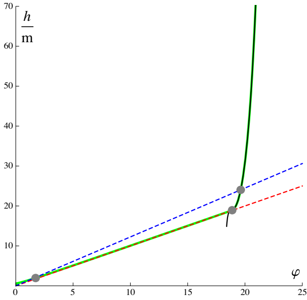
FIG. 4. The green line shows the rescaled numerical solution h/m = h(\varphi)/m of Eq. (16) with initial conditions [\varphi_0 = 22, h_0 = h(\varphi_0, b_{60}) \approx 200.79 \text{ m}] for the quadratic model v(\varphi) = m^2 \varphi^2 . The black line shows the KD approximation. The region between blue and red dotted lines is the inflation region. The gray dots correspond (from right to left) to \varphi_{\text{in}} , \varphi^* , and \varphi_{\text{end}} . We notice that the black line (KD approximation) overlaps the green line (numerical approximation) for \varphi \in (\varphi^*, \varphi_{\text{in}}) , while the red dashed line (SR approximation) overlaps the green line for \varphi \in (\varphi_{\text{end}}, \varphi^*) .
