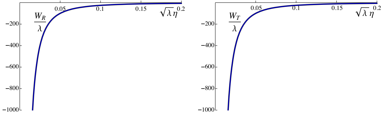
FIG. 9. Potentials W_R(\eta) (left) and W_T(\eta) (right) for the Starobinsky potential v(\varphi) = \lambda(1 - e^{-\frac{\varphi}{\sqrt{\lambda}}})^2 . The black lines show the numerical approximations, while the blue lines show the psi-series approximation [Eq. (138)]. Here we have used the rescaled variables \sqrt{\lambda}\eta , \lambda^{-1}W_R , \lambda^{-1}W_T , and the value b = \hat{b}_{60}/\sqrt{\lambda} , \hat{b}_{60} \approx 2649.03 obtained in Sec. IV A; c is taken so that a(\varphi_{\text{in}}) = 1 and \eta(t^*) = 0 in agreement with Eq. (125).
