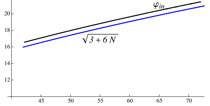
FIG. 5. The black line shows \varphi_{\text{in}} as a function of N , where \varphi_{\text{in}} is obtained from Eq. (96) and N from the formula in Eq. (97), which takes into account the contributions of both the KD stage and the SR stage. The blue line shows \varphi_{\text{in}} as a function of N as given by the SR approximation [Eq. (98)].
