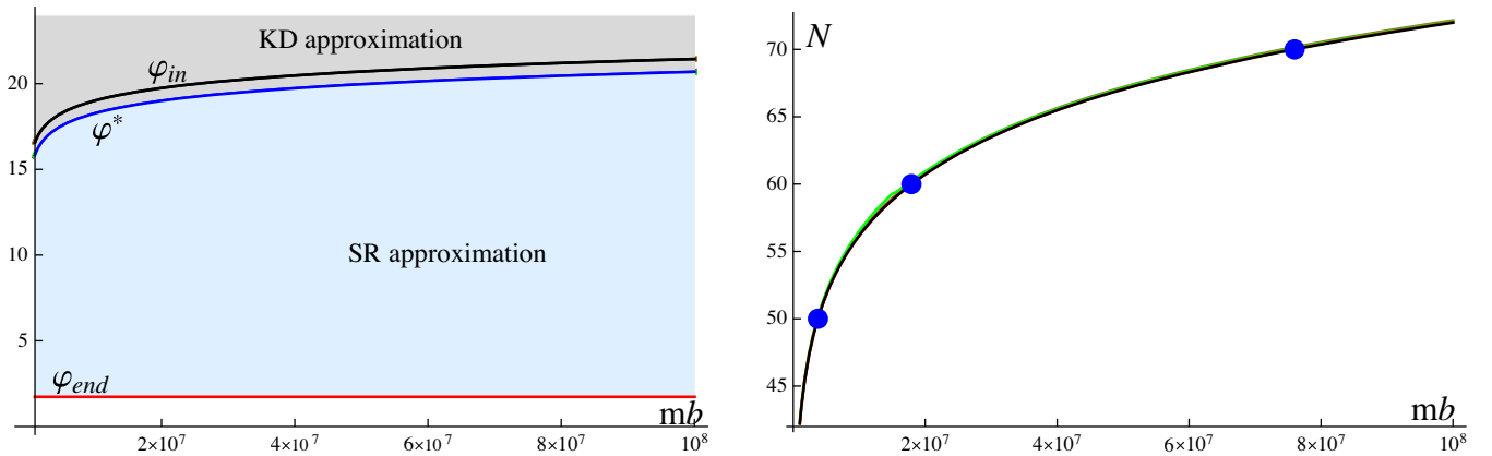
FIG. 3. The left figure shows the lines \varphi_{\text{in}}(b) (black line), \varphi^*(b) (blue line), and \varphi_{\text{end}} (red line) for the quadratic model v(\varphi) = m^2 \varphi^2 . It also shows the regions in the (mb, \varphi) plane corresponding to the KD approximation (gray region) and the SR approximation (blue region). The right figure shows the amount of inflation N(b) corresponding to the approximations with 4 (brown line), 5 (green line), 6 (red line) and 7 (black line) terms in the truncated series [Eq. (39)] provided by Eq. (97). The lines are almost completely overlapped, which shows that a very good approximation is obtained with only a few terms of the truncated series. The blue dots indicate the values N = 50, 60 , and 70 .
