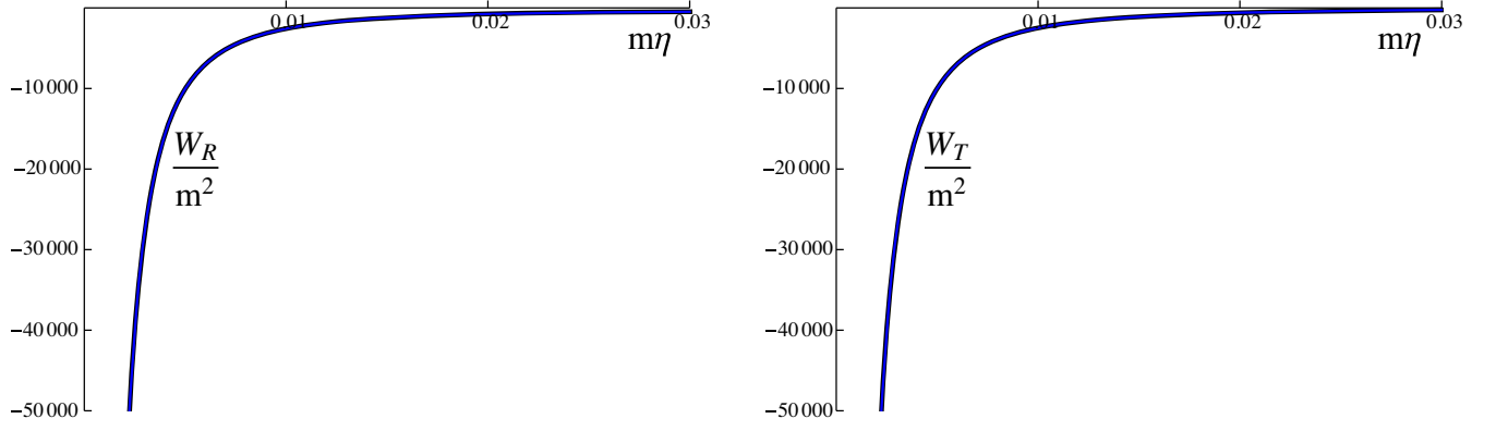
FIG. 8. Potentials W_R(\eta) (left) and W_T(\eta) (right) for the quadratic model v(\varphi) = m^2 \varphi^2 . The black lines show the numerical approximations, while the blue lines show the psi-series approximation [Eq. (121)]. Here we have used the rescaled variables m\eta , m m^{-2} W_R , m^{-2} W_T , the value b = b_{60} = \hat{b}_{60}/m , \hat{b}_{60} \approx 1.79104 \times 10^7 obtained in Sec. IV A for the quadratic model, and c is such that a(\varphi_{\text{in}}) = 1 . We have taken a value \eta(t^*) = 0 of the conformal time in agreement with Eq. (108).
