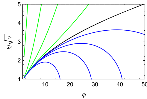
FIG. 5. Unbounded separatrix h_s(\varphi) = \varphi/\sqrt{2\varphi - 1} (black curve) and a few trajectories in \mathfrak{R}_0 for the potential v(\varphi) = (2\varphi - 1)e^{2\varphi}/\varphi^4 of Eq. (65).
