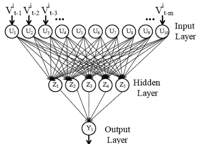
Fig. 2. Architecture of 3-Layer ANN1.
