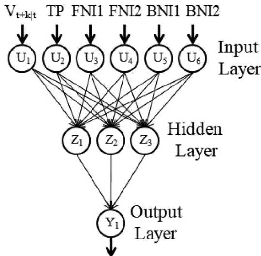
Fig. 3. Architecture of 3-Layer ANN2.
