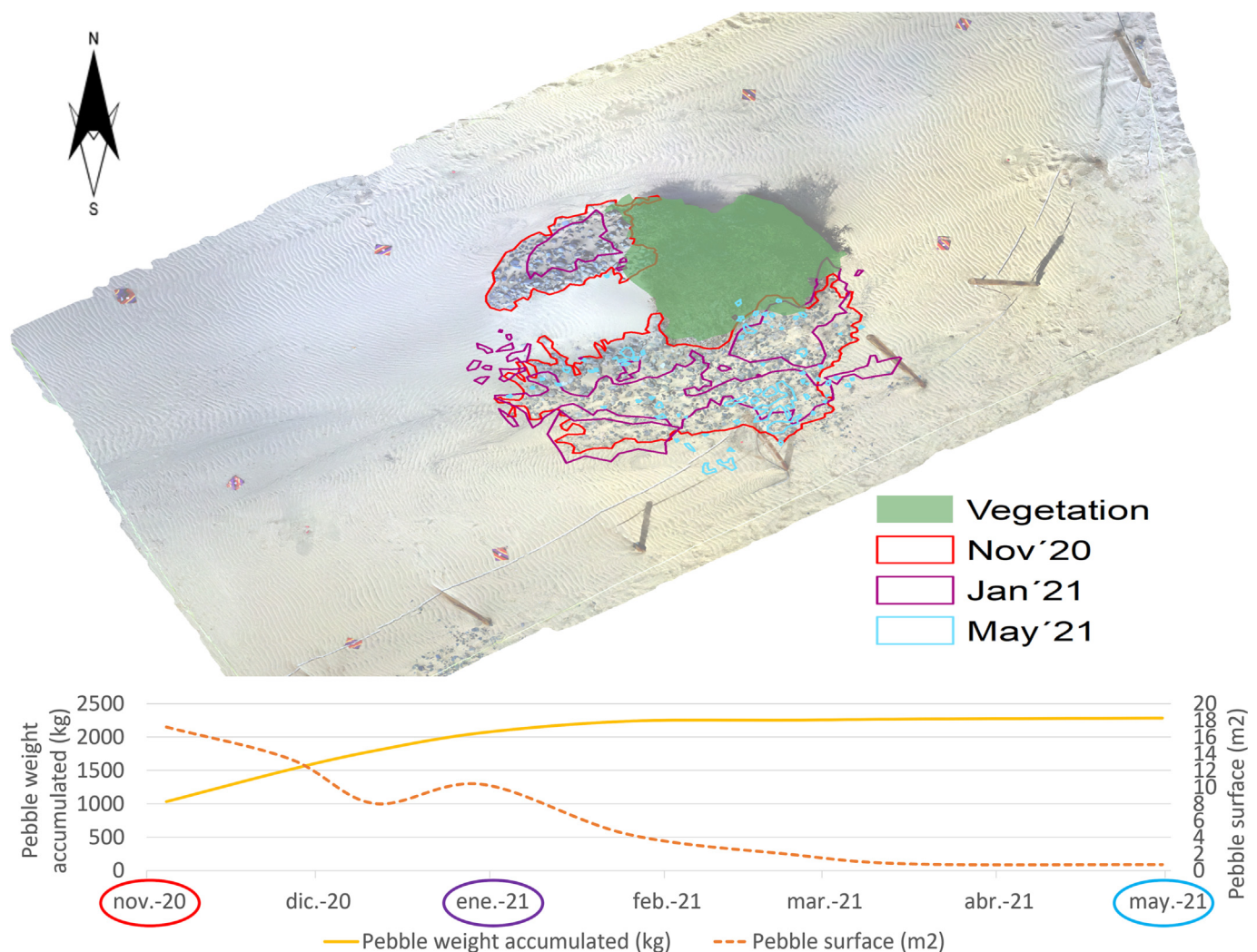
Fig. 7. Spatial evolution of surface covered by pebbles in initial (Nov'20), intermediate (Jan'21), and final (May'21) states of the experiment. The base map is an example of the ortho-mosaics obtained using Structure from Motion (FM) photogrammetry.
