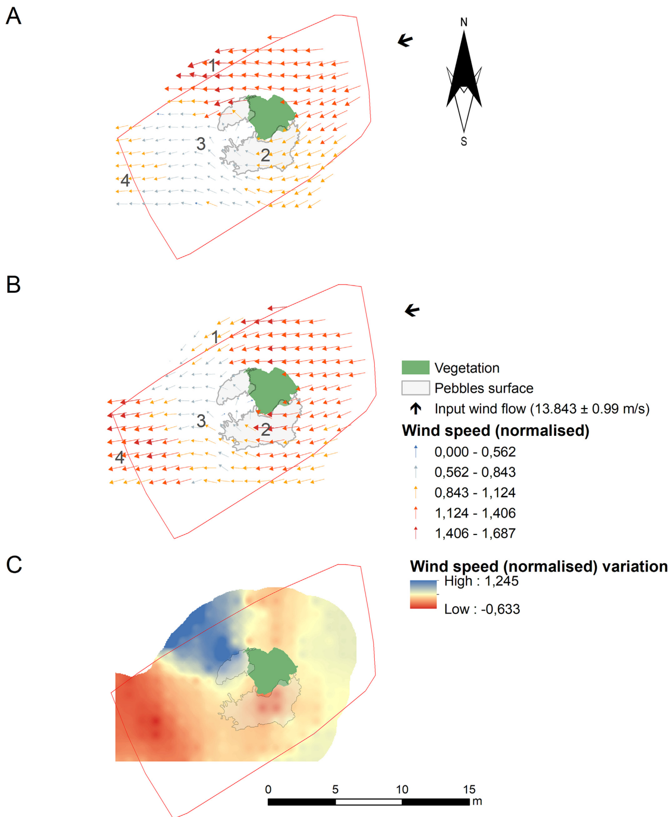
Fig. 9. Streamline distribution around the nebkha before pebble removal (A) and after pebble removal (B). Differences in wind speed after pebble removal (C). Input wind flow speed = 13.843 \pm 0.99 m/s; Input wind flow direction = 78.984 \pm 5.324^\circ .
