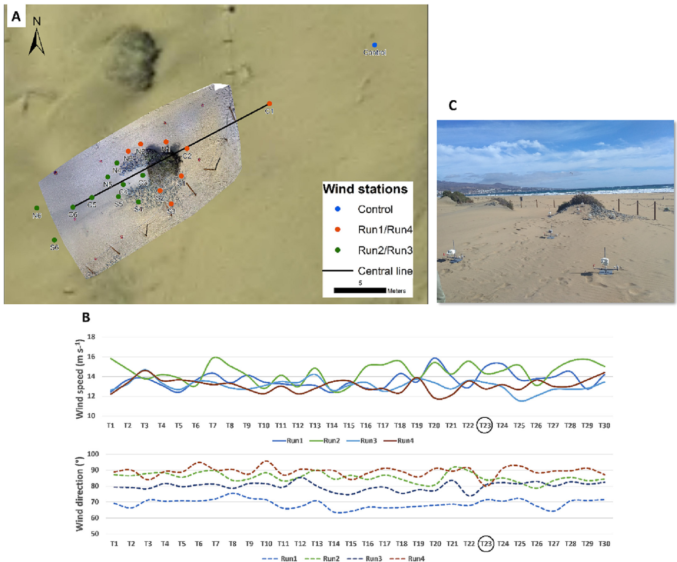
Fig. 4. A) Deployment array of sampling points around the study area. B) Temporal series of wind speeds and directions in the control station for Run 1 (STARTING TIME: 09:48) and Run 2 (STARTING TIME: 10:33), prior to the removal of the goro, and for Run 3 (STARTING TIME: 11:20) and Run 4 (STARTING TIME: 11:49) following the removal of the goro. C) Anemometers deployed around the nebkha during the field experiment.
