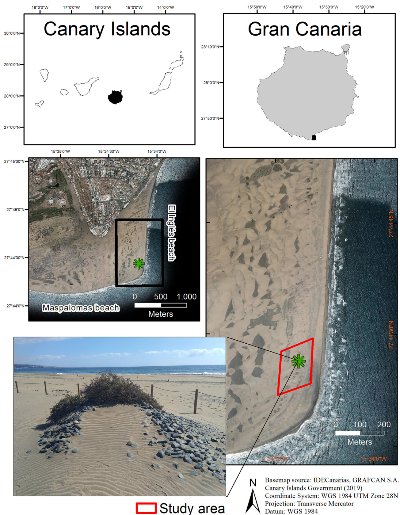
Fig. 1. Location of the study area in Playa del Inglés beach and detail of the studied stone wind shelter structure (goro) built over a nebkha (green asterisk) before the study period.
