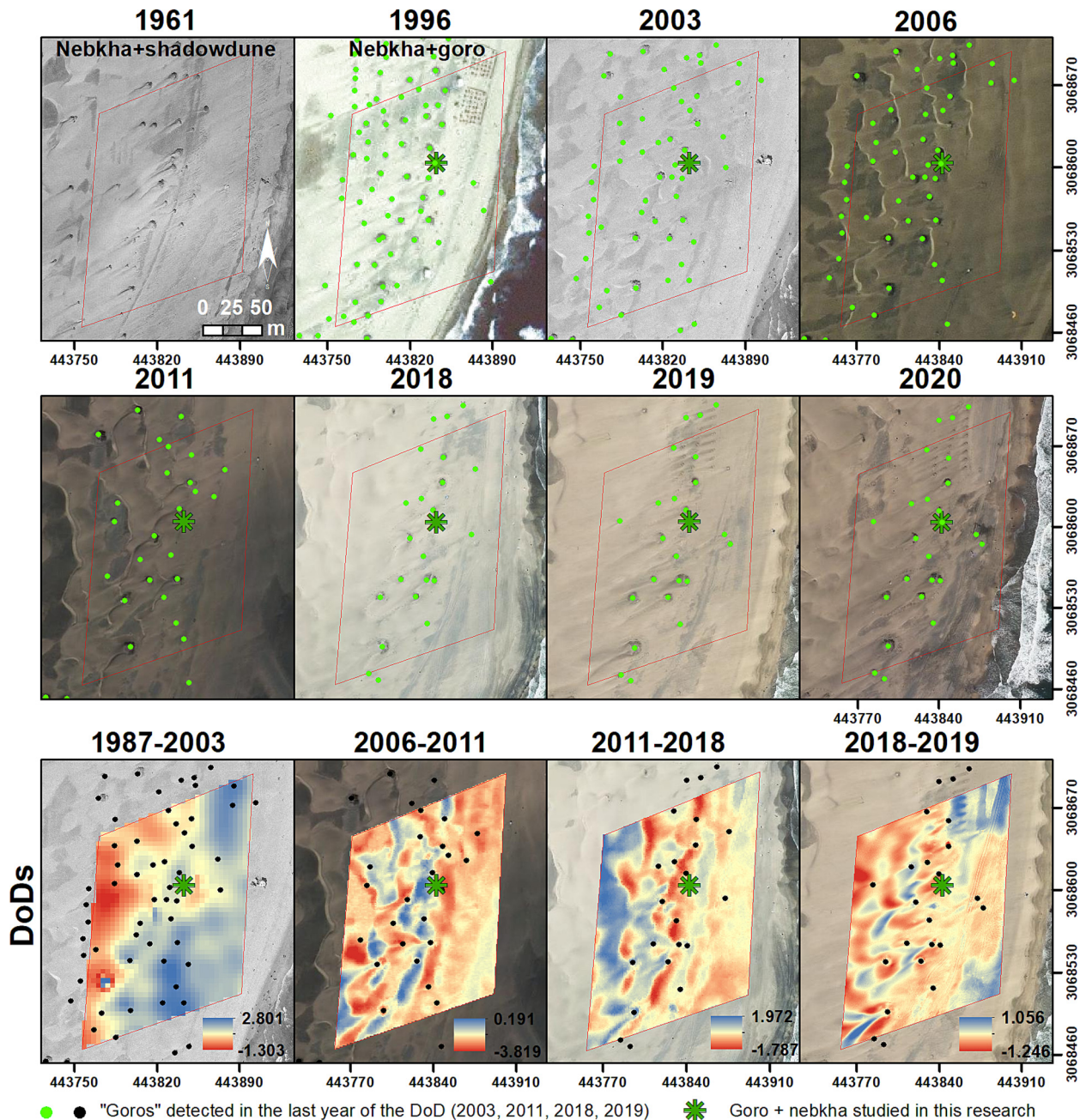
Fig. 5. Long term evolution of the study area in Playa del Inglés beach. Top: Visual evolution of the study area and goros detected from 1961 to 2020. Bottom: Topographic evolution over 32 years (1987–2019) obtained through DoDs. DoDs dates for comparison have been selected according to the limitations derived from DEMs spatial resolution (see Table 1) (Orthophotos source: SDI Canarias – Canary Islands Government-Grafcan S.A.)
