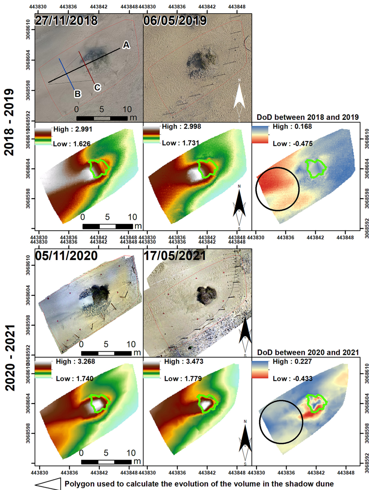
Fig. 6. Initial (left column) and final (second column) states of the nebka during the study periods. Right column shows DoDs between initial and final states, where plant contour is highlighted. Black circle marks the potential zone for shadow dune formation. Top-left image shows the three orthogonal profiles drawn for topographic monitoring (A, B, and C) and the triangular polygon used to calculate the volume of the potential shadow dune.
