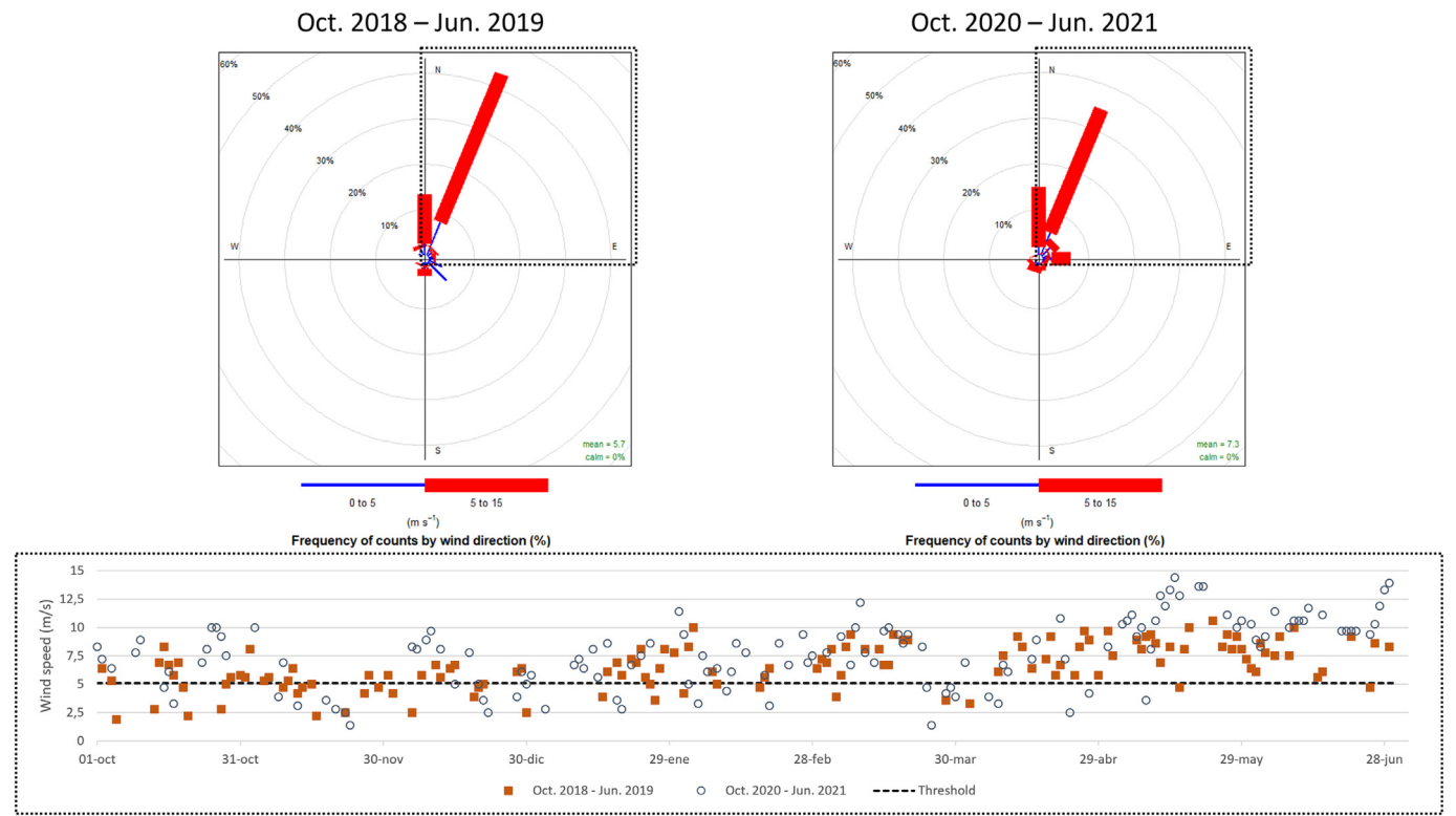
Fig. 3. Wind variability in Gran Canaria Airport (LPA). The graphics at the bottom shows only wind events from the first quadrant.
