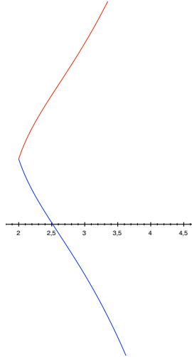
Figure 2: Red: 1 + \left( \frac{4}{1 + \tan(\frac{\pi}{\alpha})} \right)^{\frac{\alpha}{2}} Blue: 1 - \left( \frac{4}{1 + \tan(\frac{\pi}{\alpha})} \right)^{\frac{\alpha}{2}}
