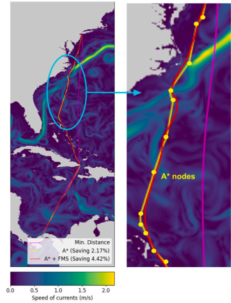
Fig. 5. Routes from New York to Panama, departing on January 1, 2023, at a sailing speed of 6 knots. The left panel compares the orthodromic route (purple), the route generated by the A* algorithm (yellow), and the optimized route produced by HADAD (red). The HADAD route demonstrates how applying the FMS algorithm smooths out the ‘jagged’ turns of the A* route, transitioning from the discrete grid-based path to a continuous trajectory. The right panel zooms in to highlight the effect of the A* grid on the jagged turns, showing how the route connects the graph nodes (marked with yellow dots).
