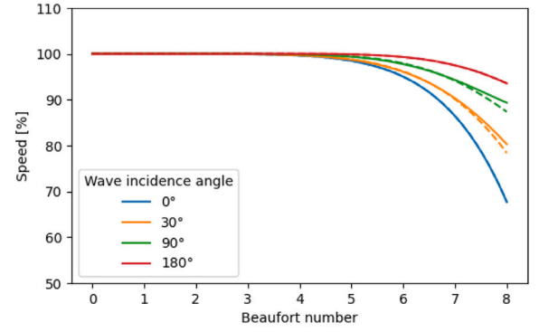
(a) Speed loss as a function of the Beaufort number, at different wave incidence angles. The smooth function closely approximates the original while eliminating discontinuities.
