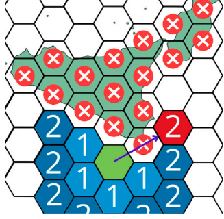
Fig. 3. The representation demonstrates how the algorithm can jump over several neighboring nodes, enhancing the flexibility of the route. Numbers on each node indicate the K -order of that neighbor to the origin (green node). It also shows the two techniques to ensure land avoidance: hexagons located directly on land are removed (marked with “x”), and edges that cross land are also removed (see the arrow connecting to the red node).
