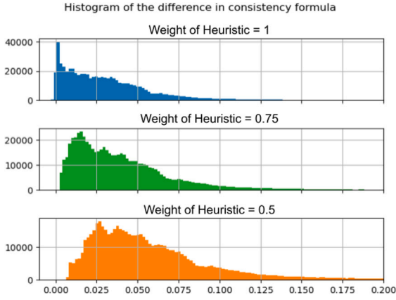
Fig. 4. Histogram of the distribution of \Delta h values for different weights of the A* heuristic, across 20 different routes, resulting in 614,494 evaluations. A consistent heuristic is one that ensures \Delta h(N) \geq 0, \forall N . As the weight of the heuristic decreases, the distribution shifts right, indicating an increase in the consistency of the heuristic.
