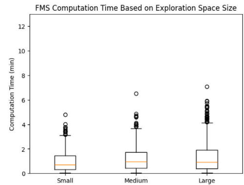
(c) Computation time of FMS for varying sizes of the exploration space. This reflects a linear behavior following O(|V|) complexity.
