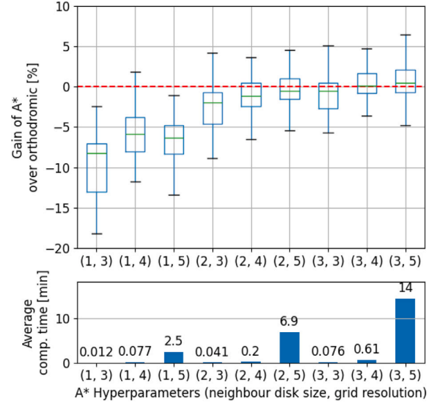
Fig. 17. Parameter settings for A*, grouped by K-order neighbors and grid resolution as defined by the H3 library (Uber Technologies, Inc., 2018). The gain of A* over orthodromic navigation is shown, and computation times are plotted below.
