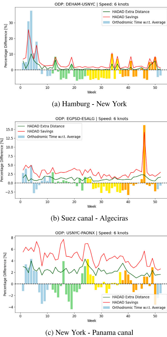
Fig. 8. Percentage difference between the orthodromic route per week to yearly average, and HADAD compared to orthodromic with respect to time and distance. Each week is colored by season, starting with winter (1st January, 2023).
