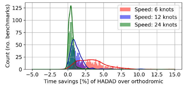
Fig. 6. Time savings of our HADAD algorithm compared to the orthodromic route. Histogram and best-fit KDE univariate distribution for each sail speed.
